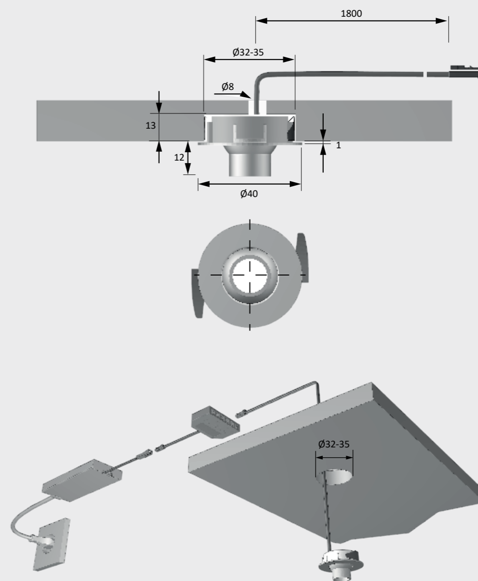
Dimensional drawing / installation
